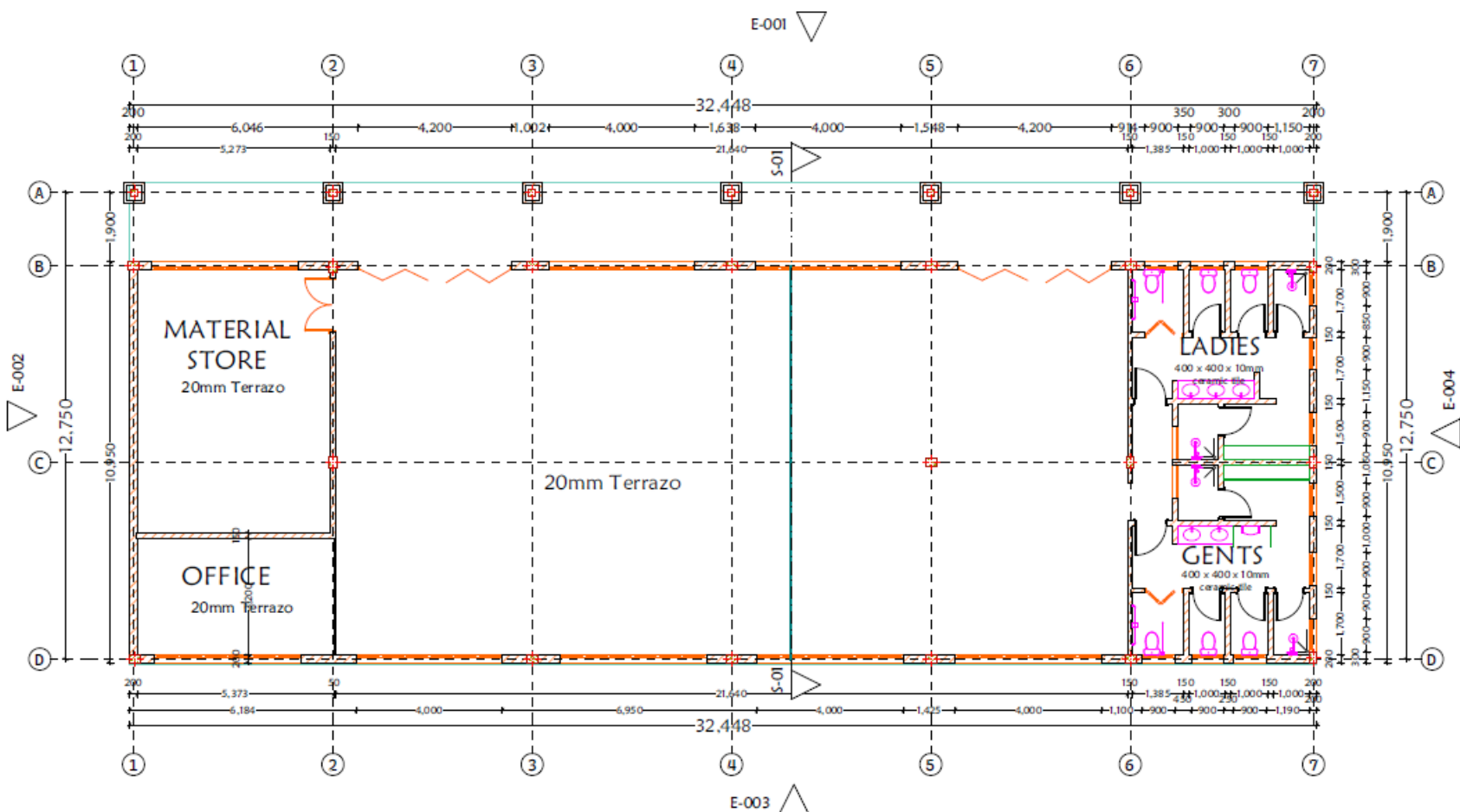
EXHIBITION WAREHOUSE FLOOR PLAN SCALE 1:100
